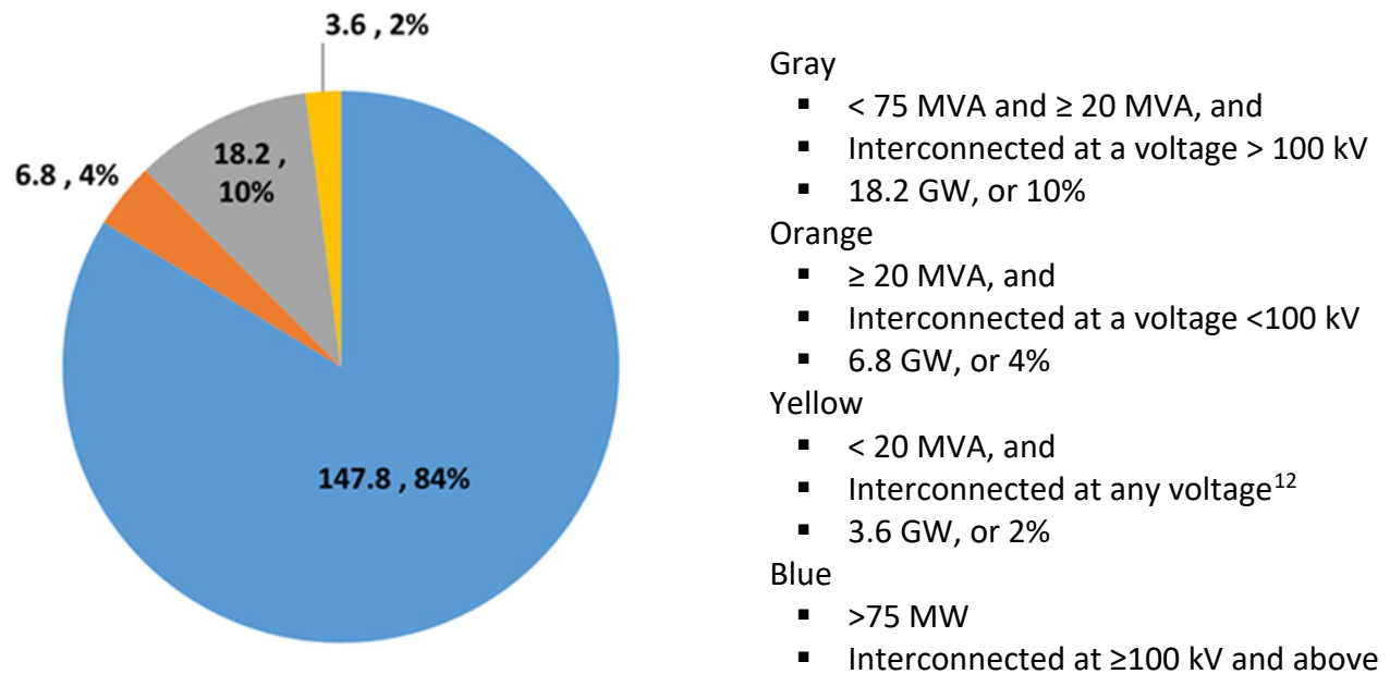
Figure 1: Percent shares of BPS-connected IBRs by aggregate nameplate capacity
